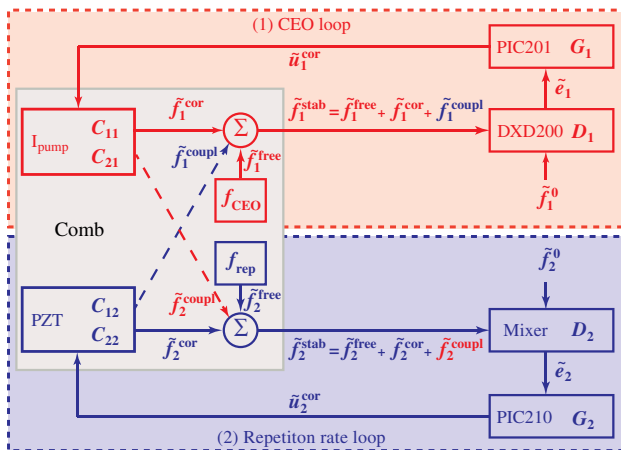
Fig. 3. (Color online) Schematic representation of the two coupled stabilization loops in the Er: fiber comb. Loop (1) stabilizes the CEO frequency and loop (2) the repetition rate.
